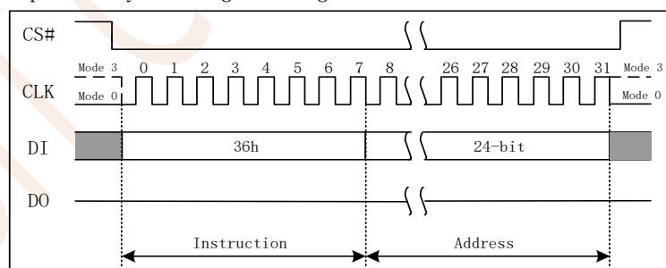
Figure 7.36 Read Manufacturer/Device ID Dual I/O Instruction
