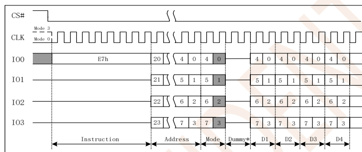
Figure 7.20 Word Read Quad I/O Instruction(Initial command or previous M5-4 ≠10)
