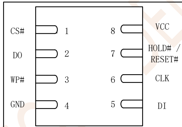
Figure 3.2 DFN8 (5*6 mm)
