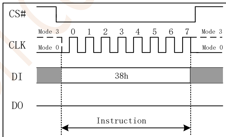
Figure 7.41 Enter QPI Instruction (SPI Mode only)
