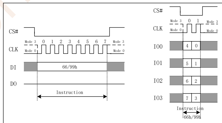
Figure 7.25 Software Reset Instruction (SPI and QPI Mode)
