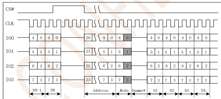
Figure 7.20 Word Read Quad I/O Instruction(Initial command or previous M5-4 ≠10)
