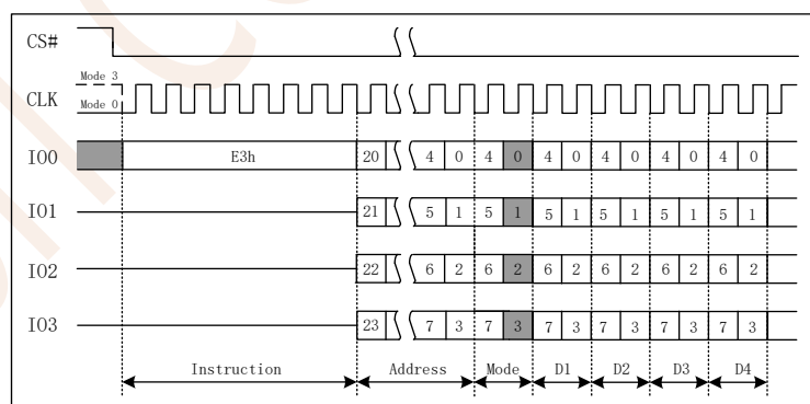
Figure 7.22 Octal Word Read Quad I/O Instruction(Initial command or previous M5-4 \neq 10)
