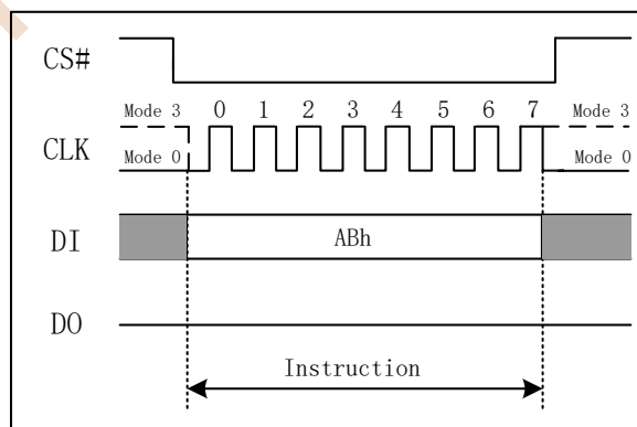
Figure 7.13 Release Power-down Instruction
