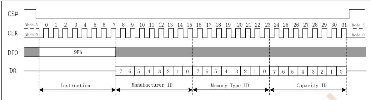
Figure 7.16 Read JEDEC ID
