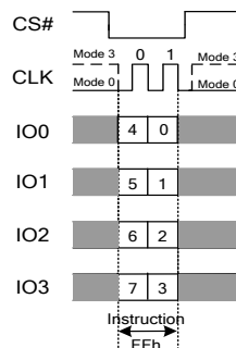
Figure 7.42 Exit QPI Instruction (QPI Mode only)
