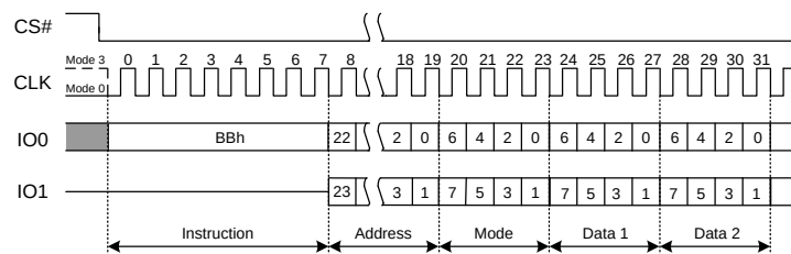
Figure 7.17 Fast Read Dual I/O Instruction (Initial command or previous M5-4#10) Sequence Diagram
