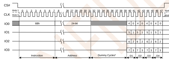
Figure 7.16 Fast Read Quad Output Instruction Sequence Diagram
