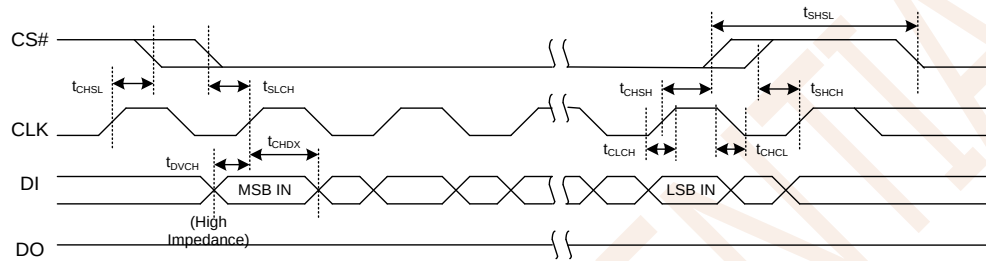
Figure 8.5 Input Timing
