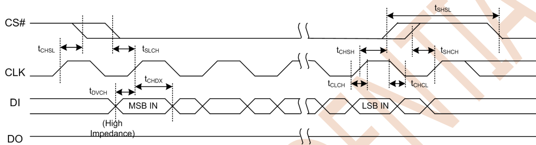
Figure 8.5 Input Timing
