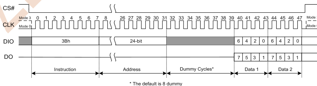
Figure 7.11 Fast Read Dual Output Instruction Sequence Diagram
