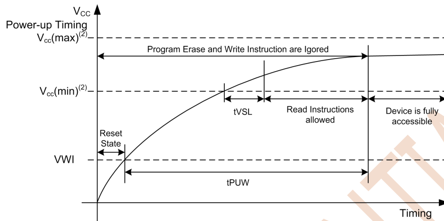
Figure 8.1 Power-up Timing
