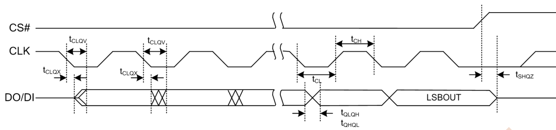
Figure 8.4 Serial Output Timing
